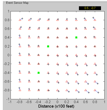
Fig. 10. Localization with anchor nodes deployed non-linearly around the center of the sensor bed.
